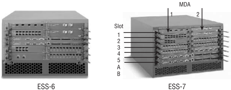
Figure 2.5 The Alcatel-Lucent 7450 ESS-7 and ESS-6. Two slots are dedicated for SF/CPM control cards for both models. The other slots are available for I/O Modules that provide network interfaces.
