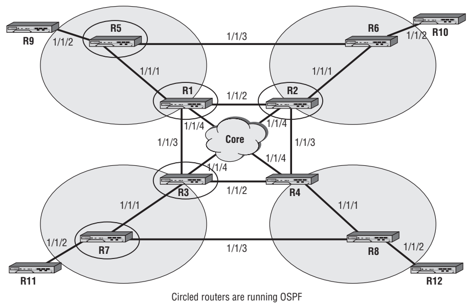
Figure 9.7 A sample network topology. For the examples that follow, only routers R1, R2, R3, R5, and R7 have been enabled for OSPF.
