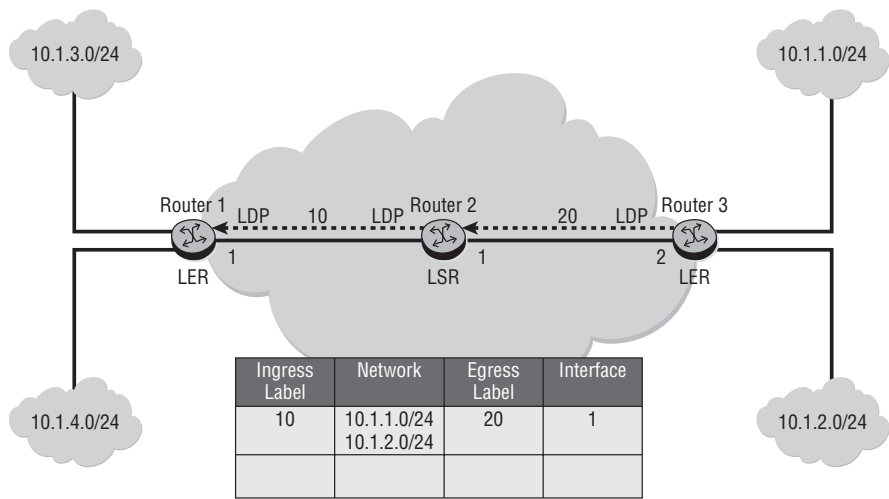
Figure 11.6: Router 2 uses LDP to update Router 1 with label information about the networks on Router 3. Router 2 sends label 10 to Router 1, so Router 1 will tag any packets with a destination address of the networks on Router 3 with a 10 tag and forward it to Router 2. Router 2 will swap the 10 tag with a 20 tag and forward the packets on to Router 3.
