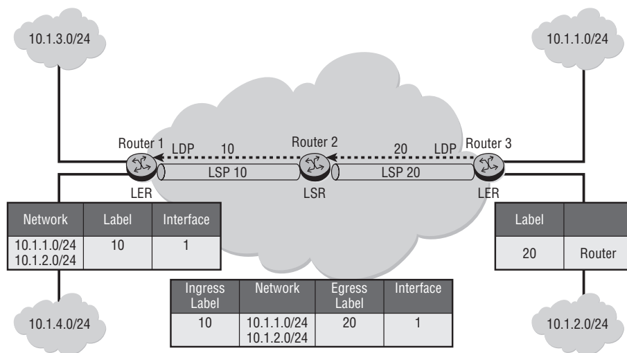
Figure 11.7: A complete tunnel is set up between Router 1 and Router 3. Router 1 is the provider ingress and will apply a 10 label to packets with a destination of 10.1.1.0/24 or 10.1.2.0/24. The packet is forwarded to Router 2 with label 10, and Router 2 swaps label 20 for label 10 and forwards it to Router 3. Router 3 pops the label from the packet and forwards the original packet to its destination CE.
